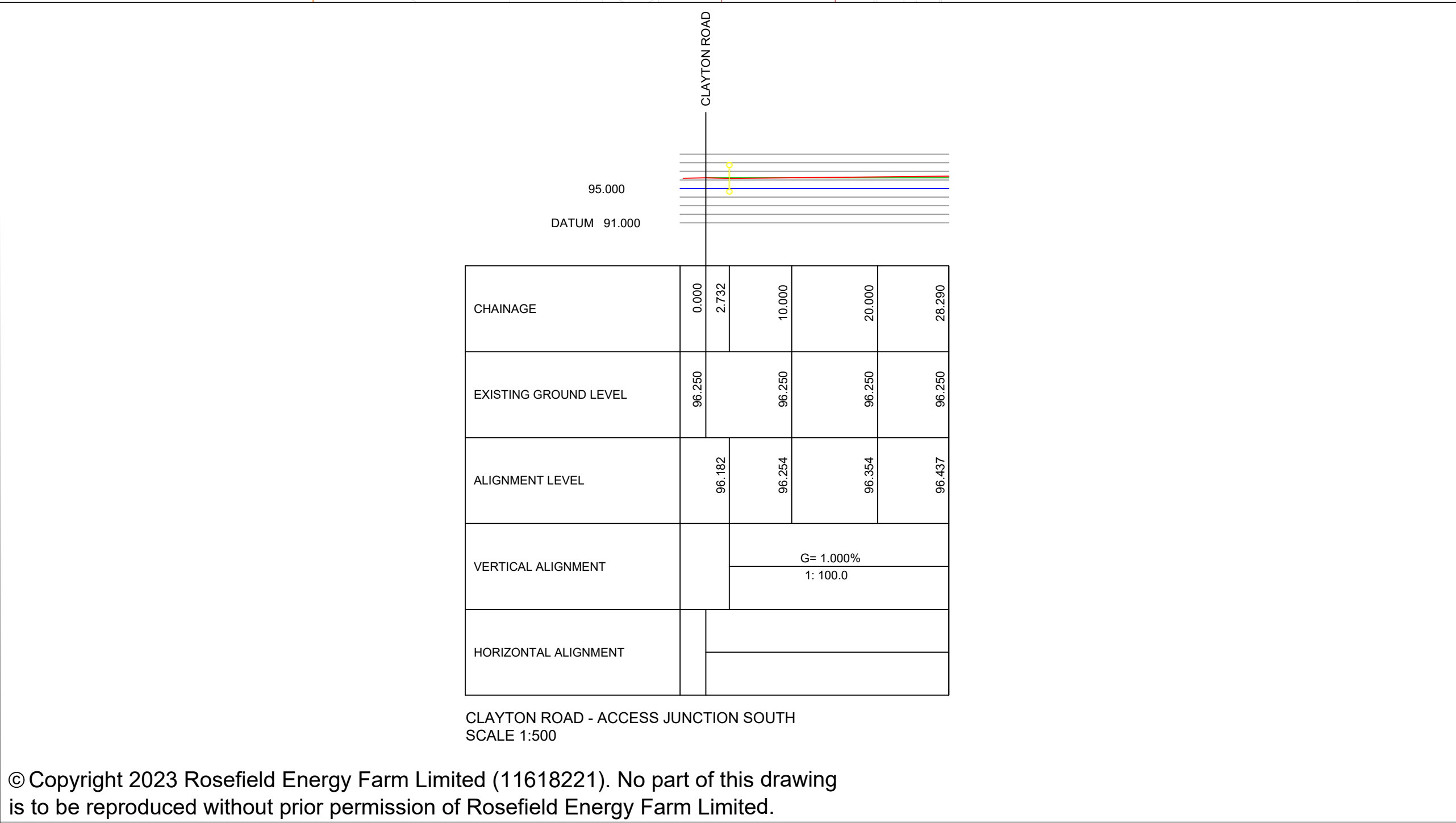
PROPOSED ACCESS JUNCTION GENERAL ARRANGEMENT SCALE 1:200
